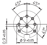
KFR 80
